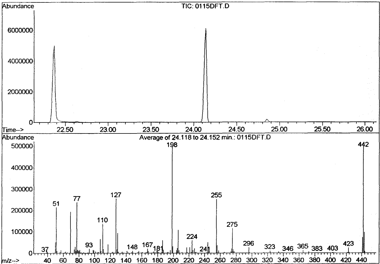
Spectrum Information: Average of 24.118 to 24.152 min.
