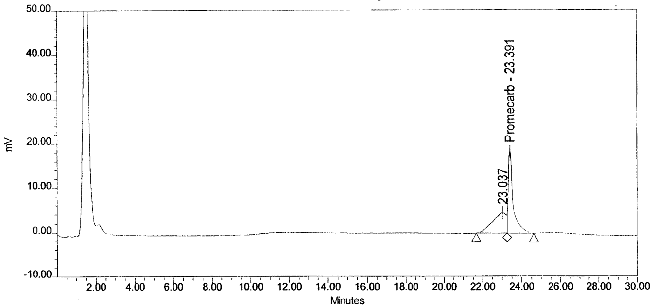
Auto-Scaled Chromatogram
