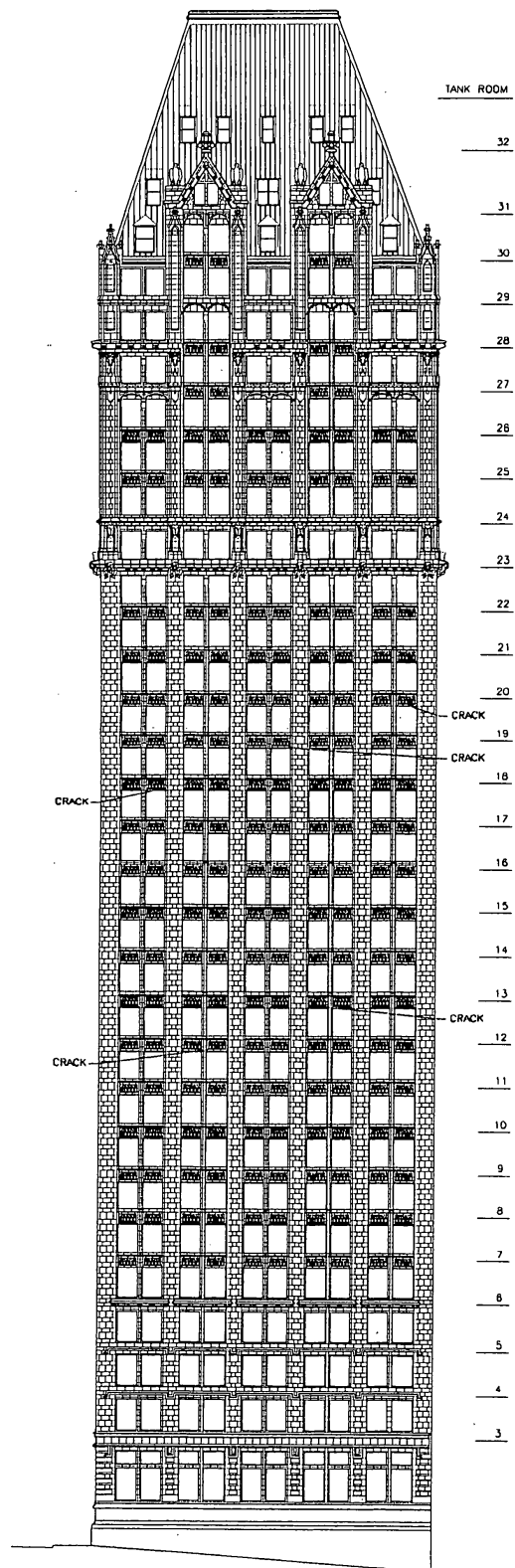
EAST ELEVATION 9/28/01
