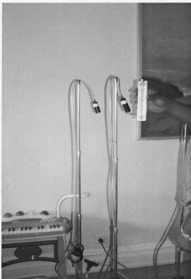
Photo 3: Calibration of Air Sampling Pumps
