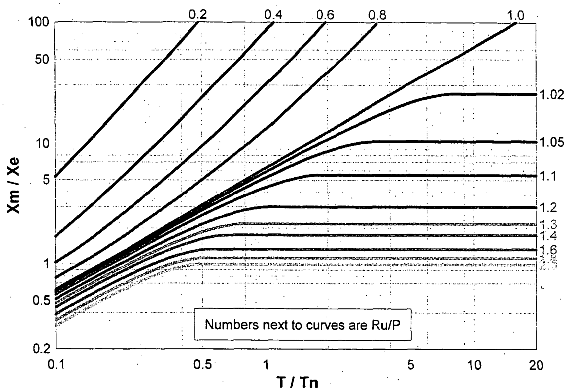
Maximum Deflection of Elasto-Plastic Single-Degree of Freedom System for Rectangular Load.
