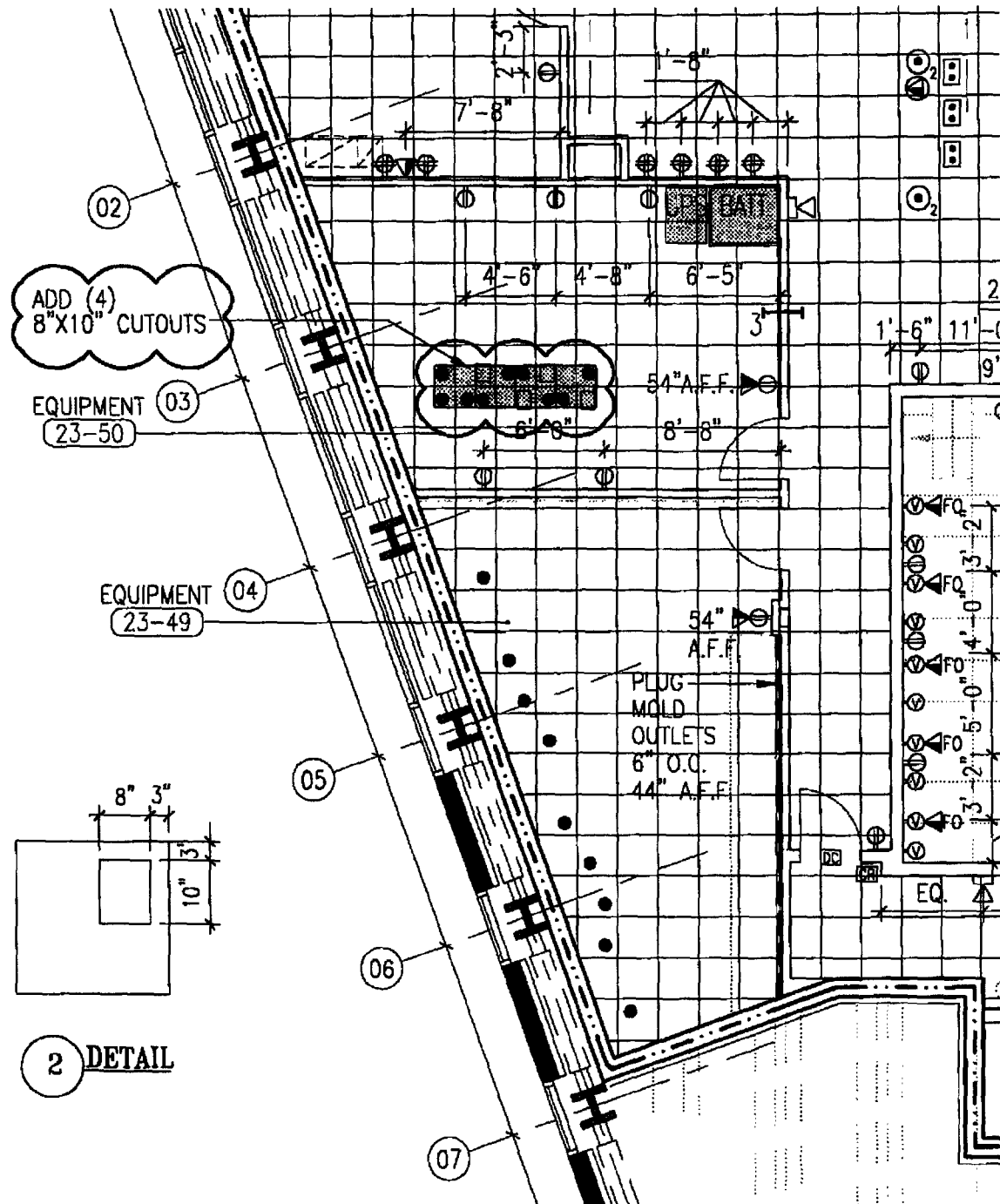
1 PART POWER PLAN RM# 23-50 & 23-49 1/8" = 1'-0"
