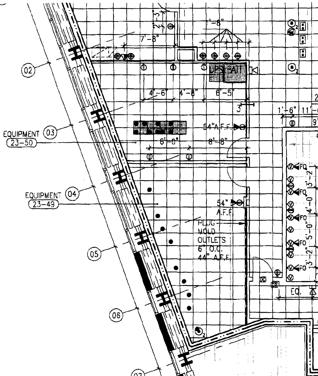
1 PART POWER PLAN RM# 23-50 & 23-49 1/8" = 1'-0"
