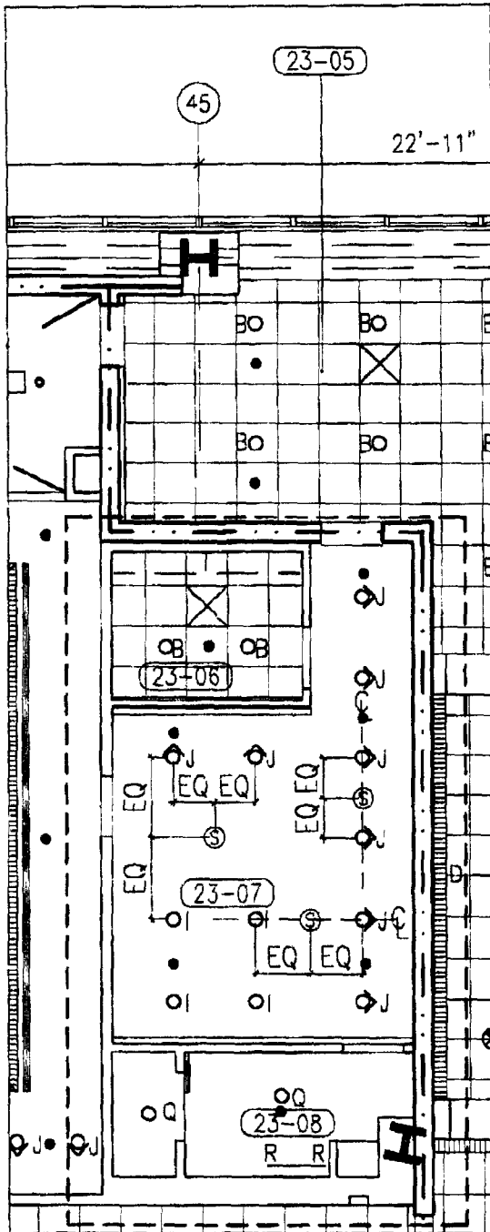
1 PART RCP RM# 23-07 1/8" = 1'-0"
