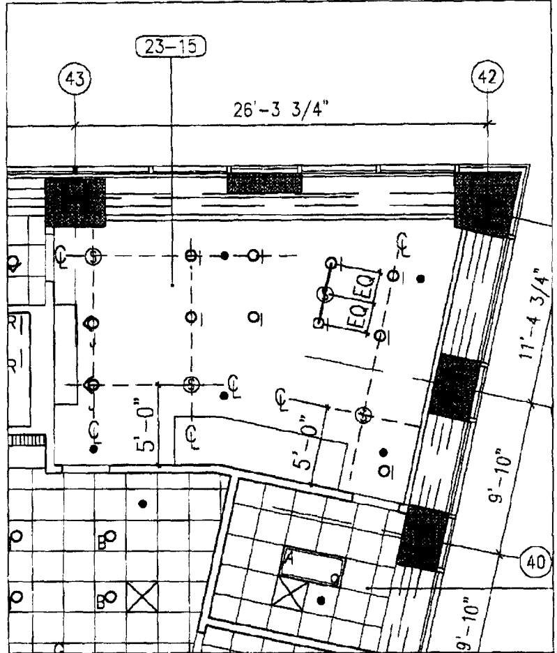
2 PART RCP RM# 23-15 1/8" = 1'-0"
