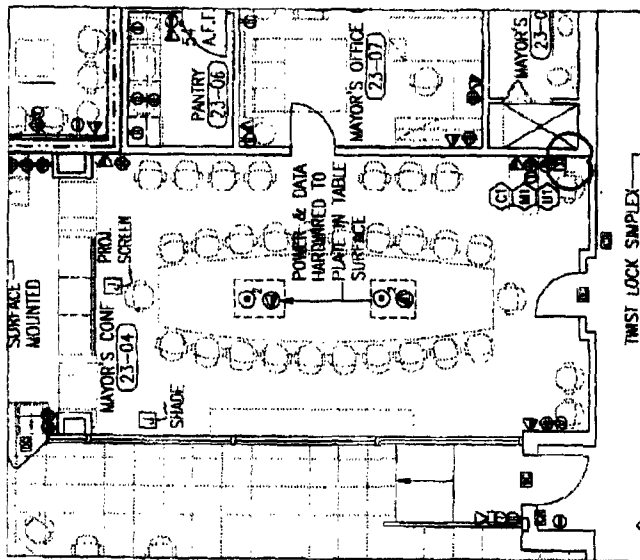
1 MAYORS CONF. ROOM 1/8" = 1'-0"
