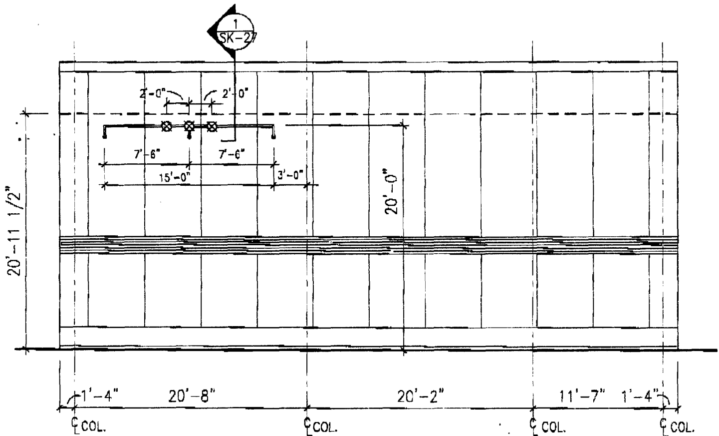
A NORTH ELEVATION @ PENTHOUSE 1/8"=1'-0"
