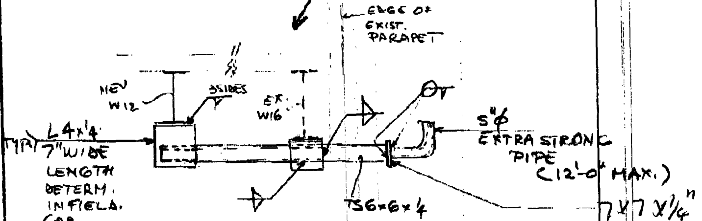
ROOF BULKHEAD FRAMING PLAN
