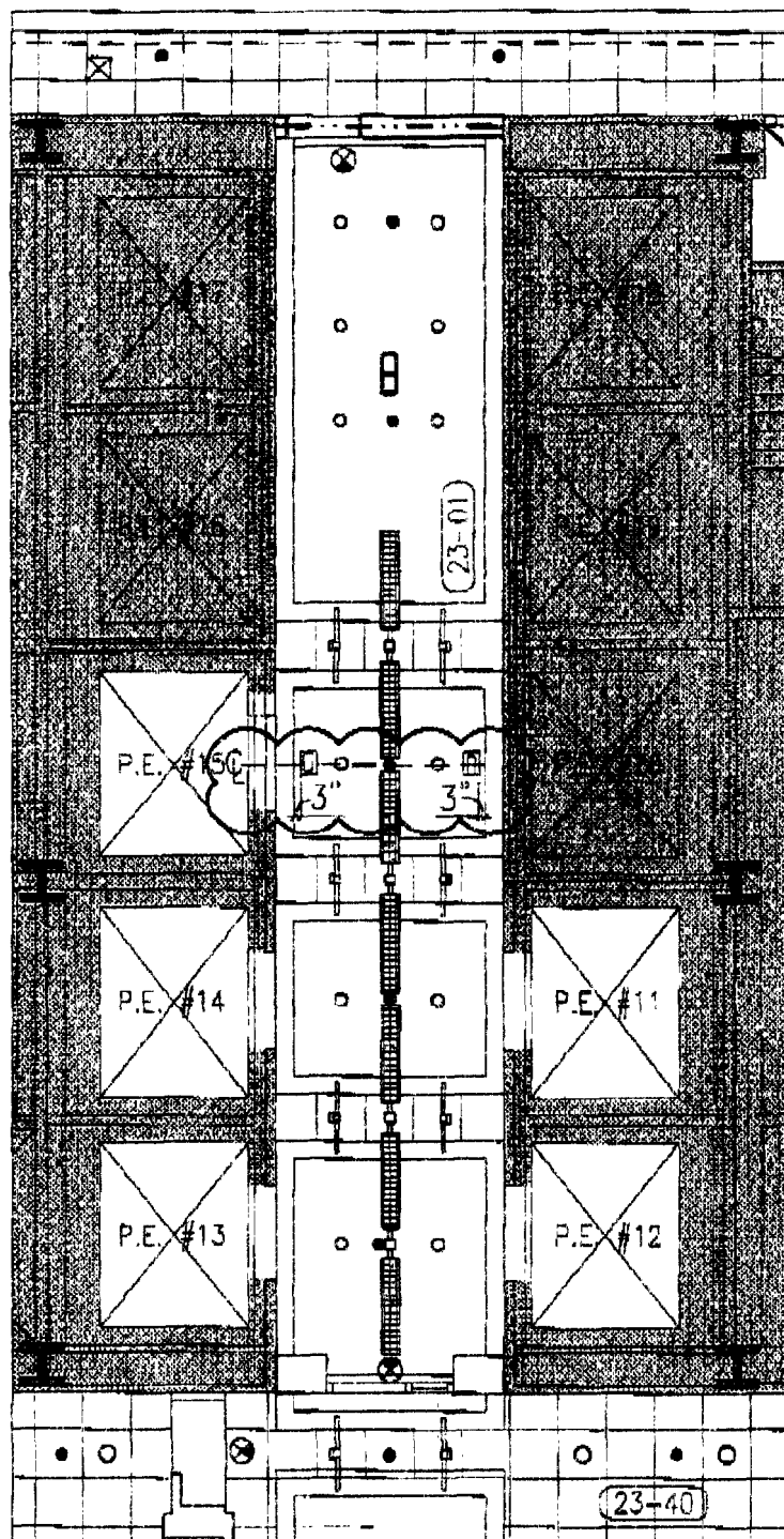
1 PART RCP PLAN 1/8"=1'-0"
