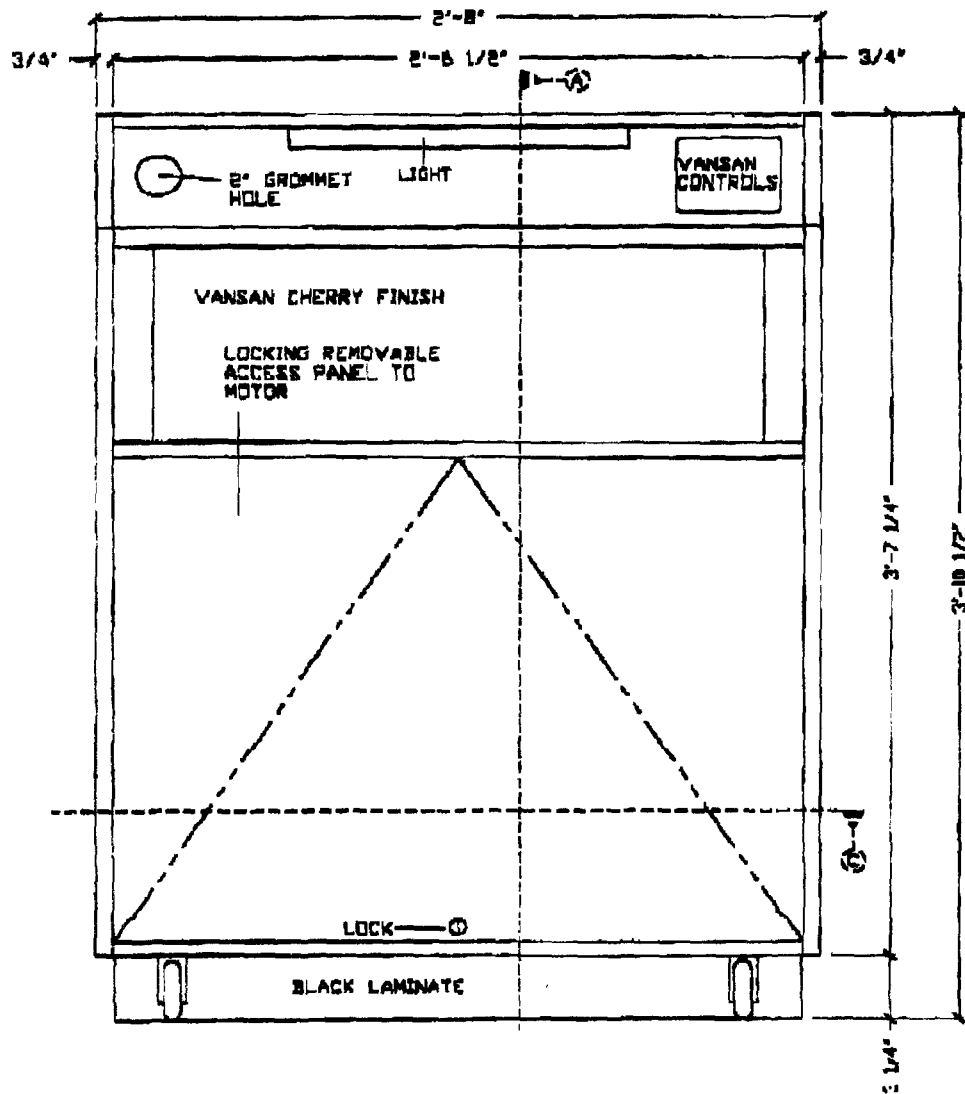
REAR ELEVATION
