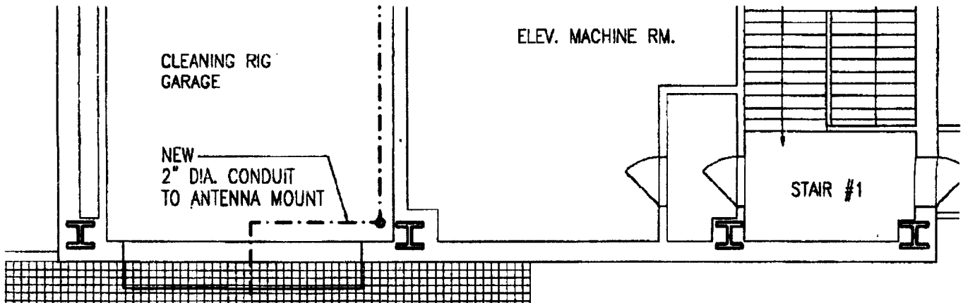
1 KEY PLAN FOR ROOF 1/8"=1'-0"
