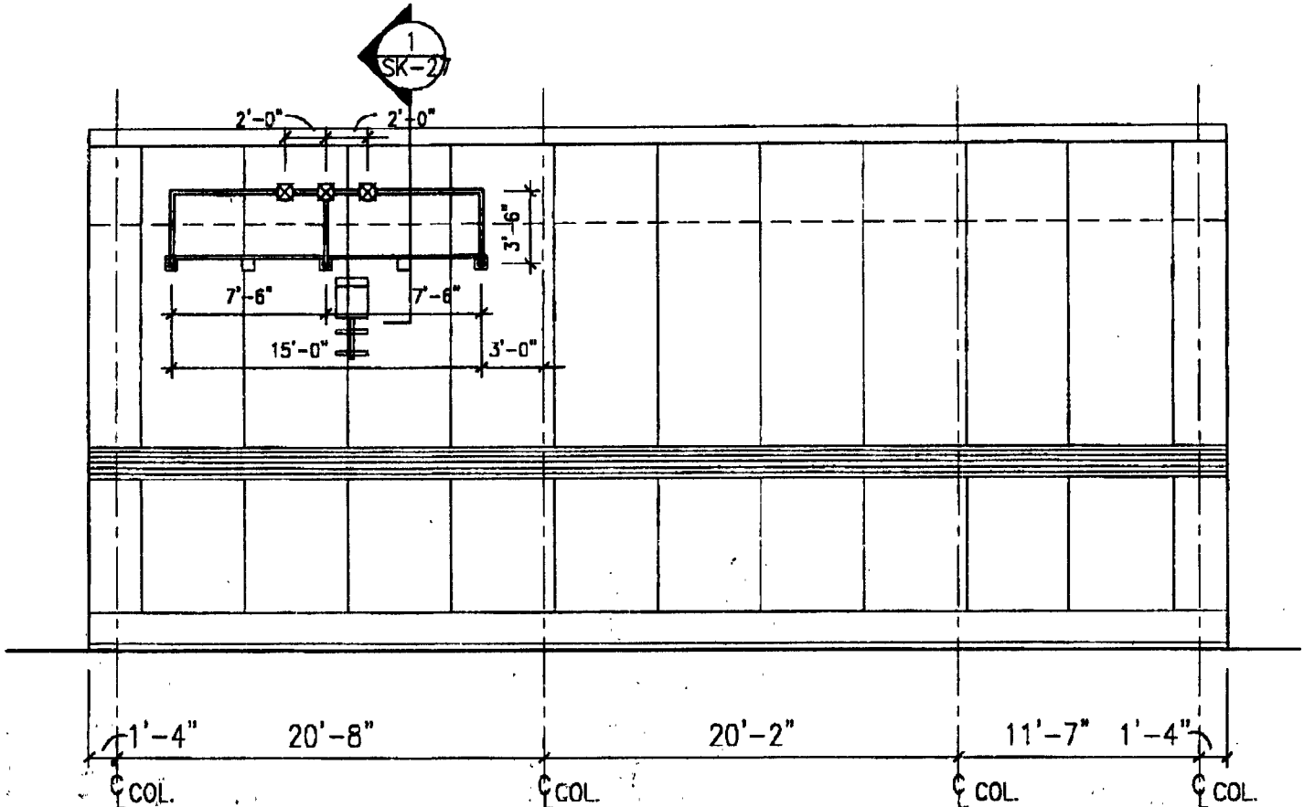
A NORTH ELEVATION @ PENTHOUSE 1/8"=1'-0"
