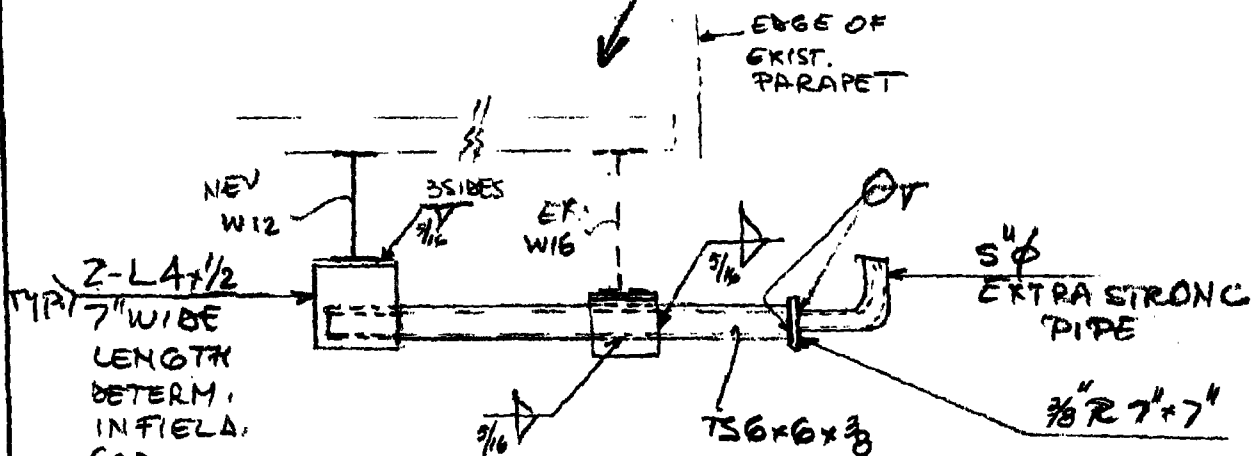
ROOF BULKHEAD FRAMING PLAN
