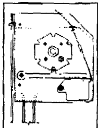
Fire Door Adjuster and Release Mechanism
