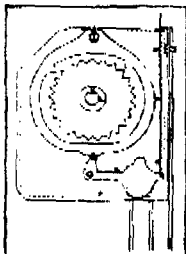
Fire Door Descent Control Mechanism (Governor)
