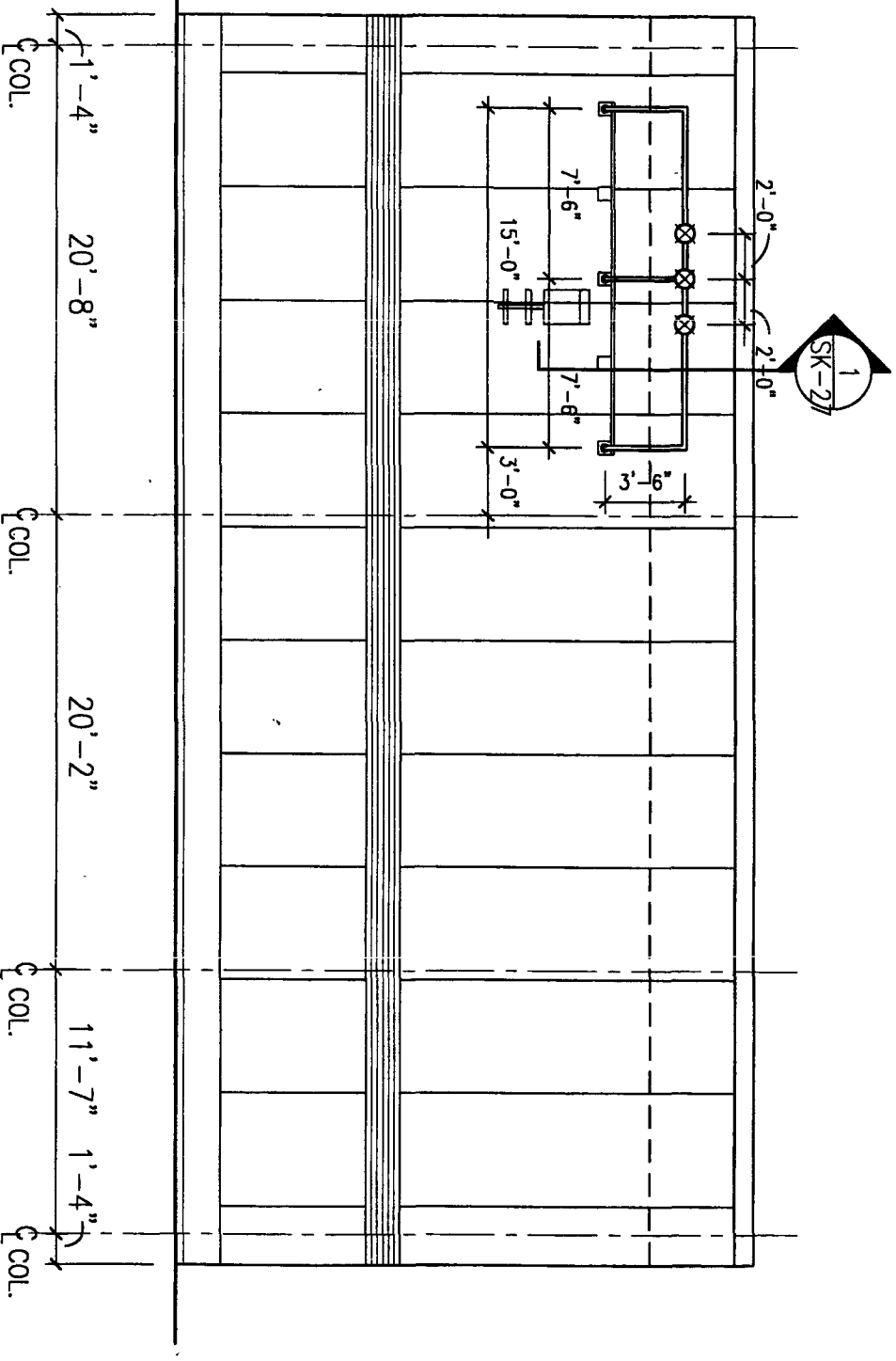
A NORTH ELEVATION @ PENTHOUSE 1/8"=1'-0"
