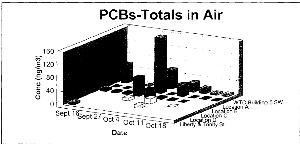
Figure 8. PCBs-Totals in Air at Six Locations.
