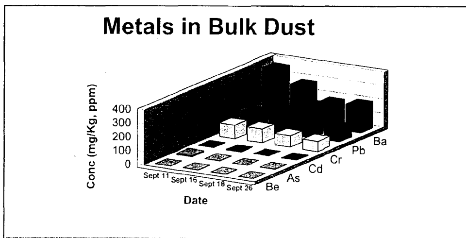
Figure 14. Metals Profile in Bulk Dust; Four Sites over Four Dates
