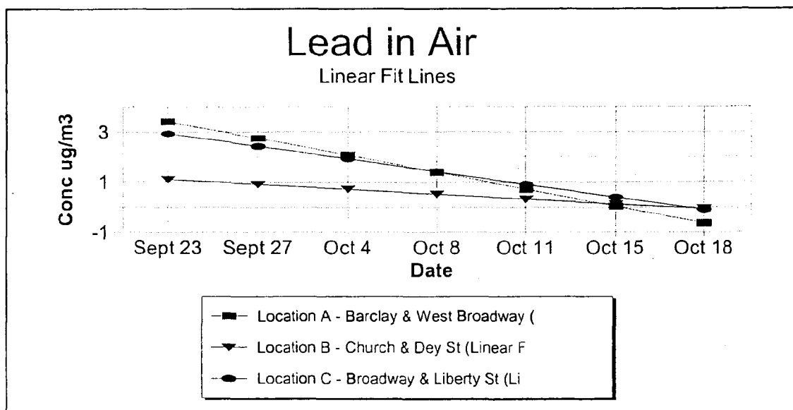
Figure 12. Linear Fitted Lines for Lead in Air at Three locations.
