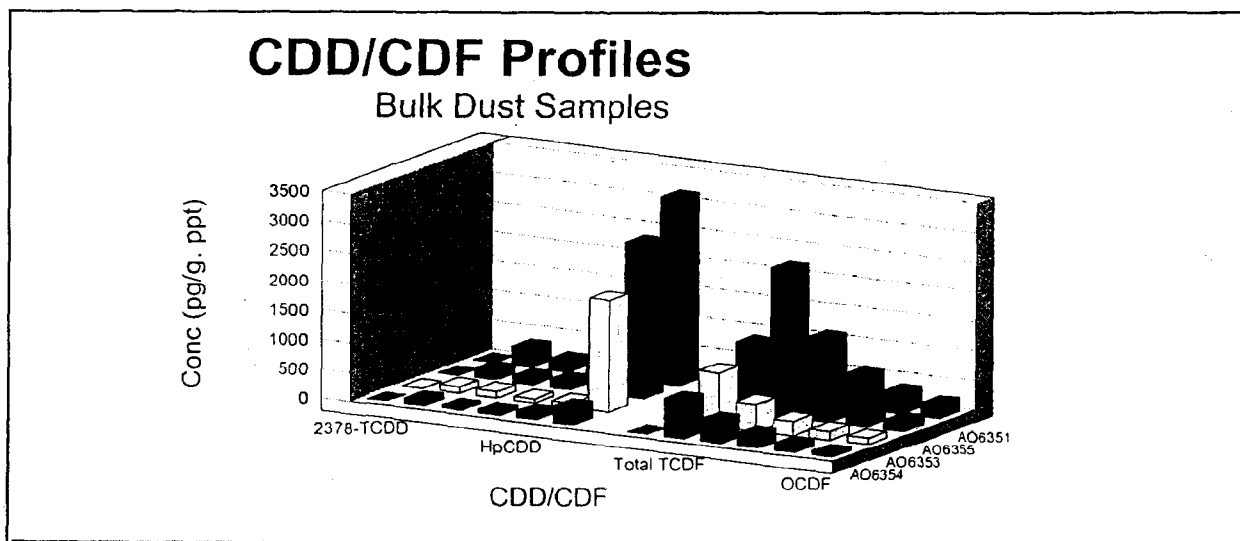
Figure 7. CDD/CDF Profile in Bulk Dust from Sept 16 th at Battery Park and 2 nd Pl.
