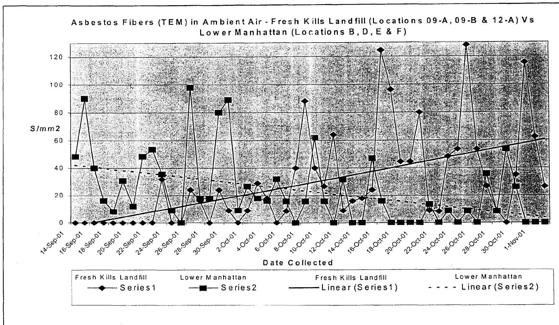
Figure 5. TEM asbestos results and fitted lines from Lower Manhattan and Fresh Kills Landfill
