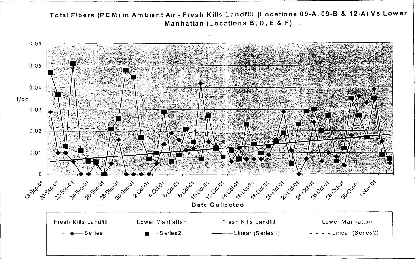
Figure 4. Total Fibers (PCM) in Ambient Air from Lower Manhattan and Fresh Kills Landfill.
